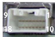
18 pin radio connector
