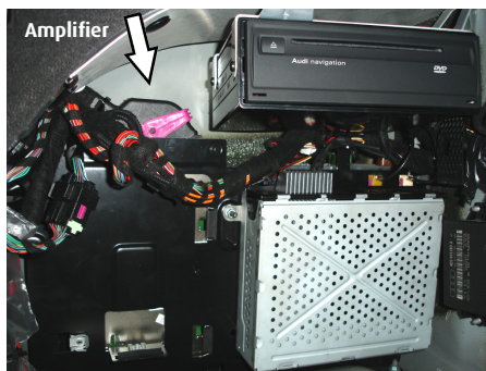
Pictures of amplifier location in Audi A8
