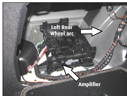
Amplifier location in Audi A4, A4 Allroad & A5
