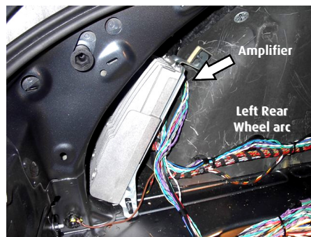
Pictures of amplifier location in Audi TT
