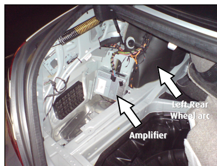
Amplifier location in S & CL-Class
