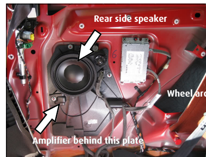
Amplifier location in Volvo C30
